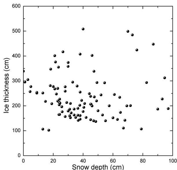
Fig. 1. Variability in snow depth and ice thickness measured at over 100 sites in mid-May.
