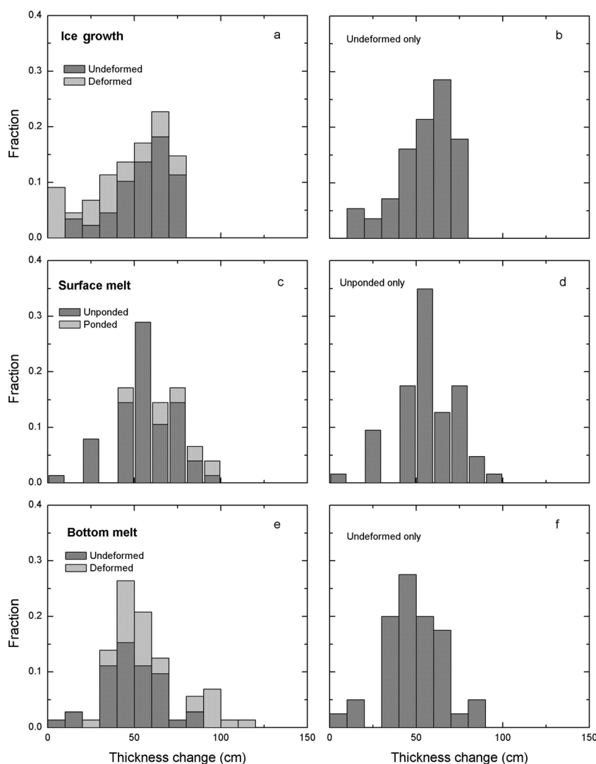
Fig. 3. Mass-balance histograms of ice growth, surface melt and bottom melt tabulated from measurements selected from 100 sites measured during the SHEBA field campaign. (a), (c) and (e) include data from all of the sites. (b), (d) and (f) only include data from sites located on undeformed and unponded ice.
