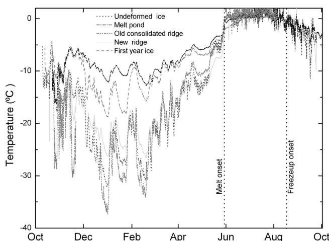
Fig. 2. The annual cycle of snow-ice interface temperatures measured at five locations during the SHEBA field program.
